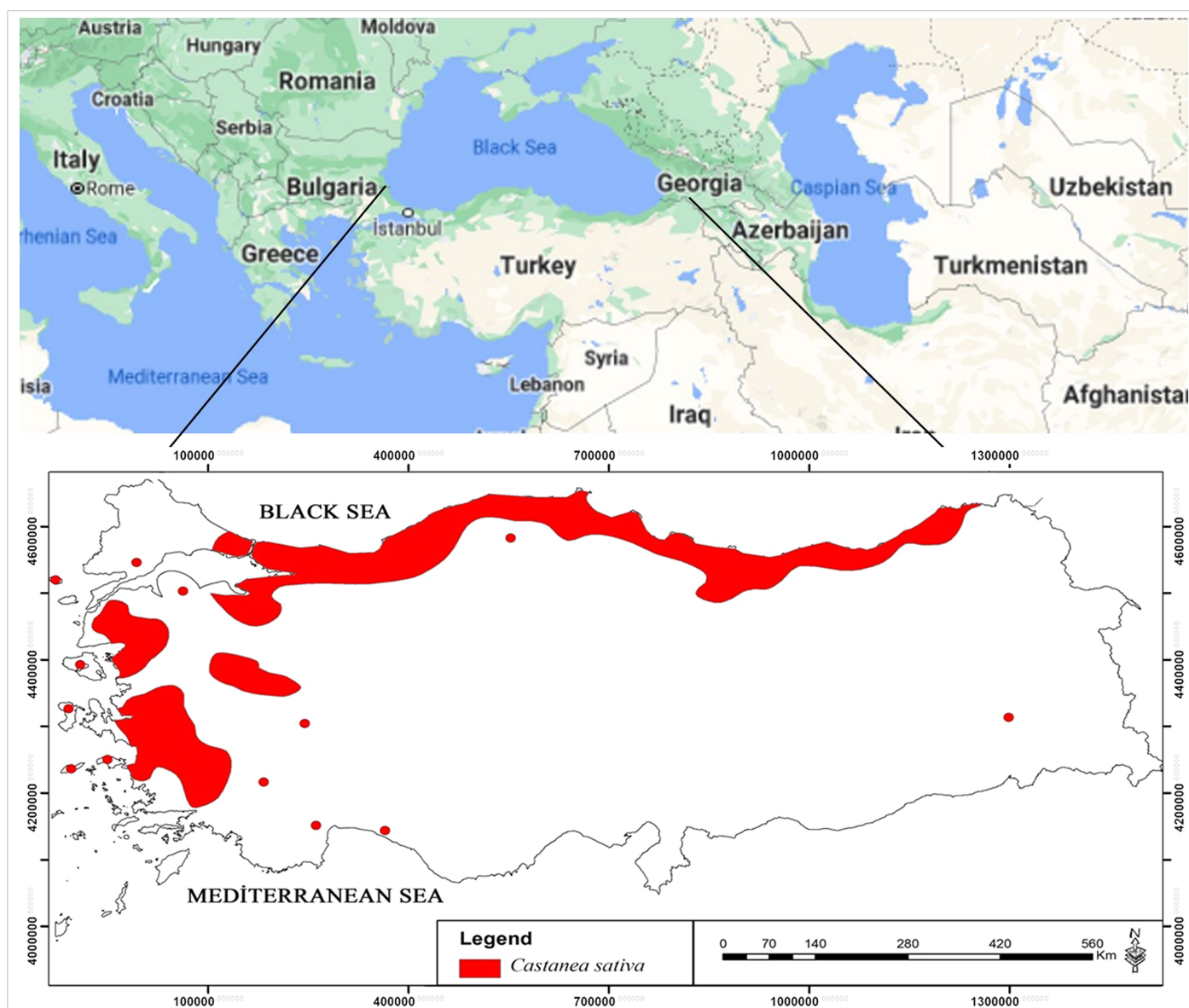
Figure 1. Current (2020) Distribution Area of Anatolian Chestnut ( Castanea sativa ) in the Study Boundary.
